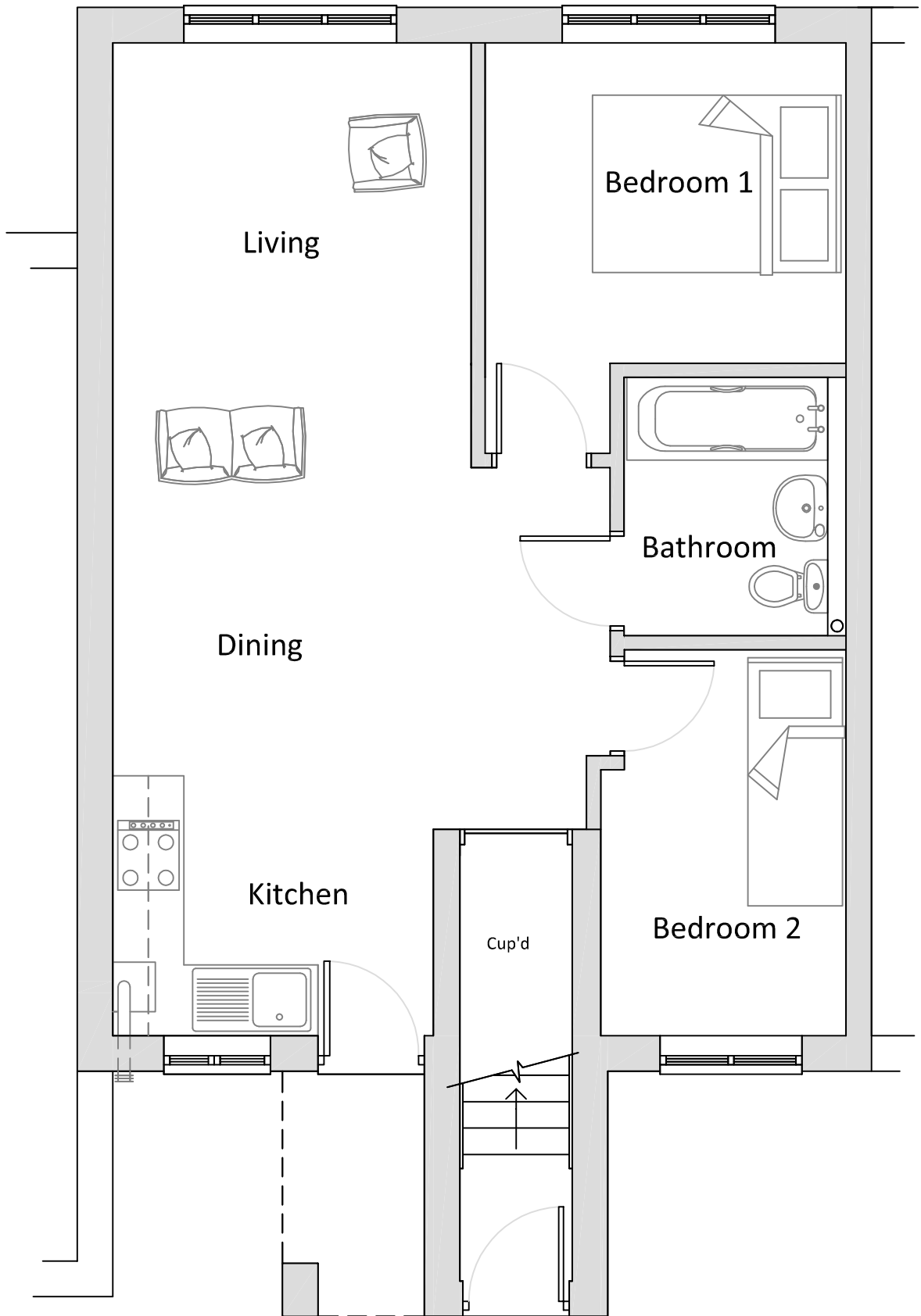
Ground Floor Layout Flat No 7
