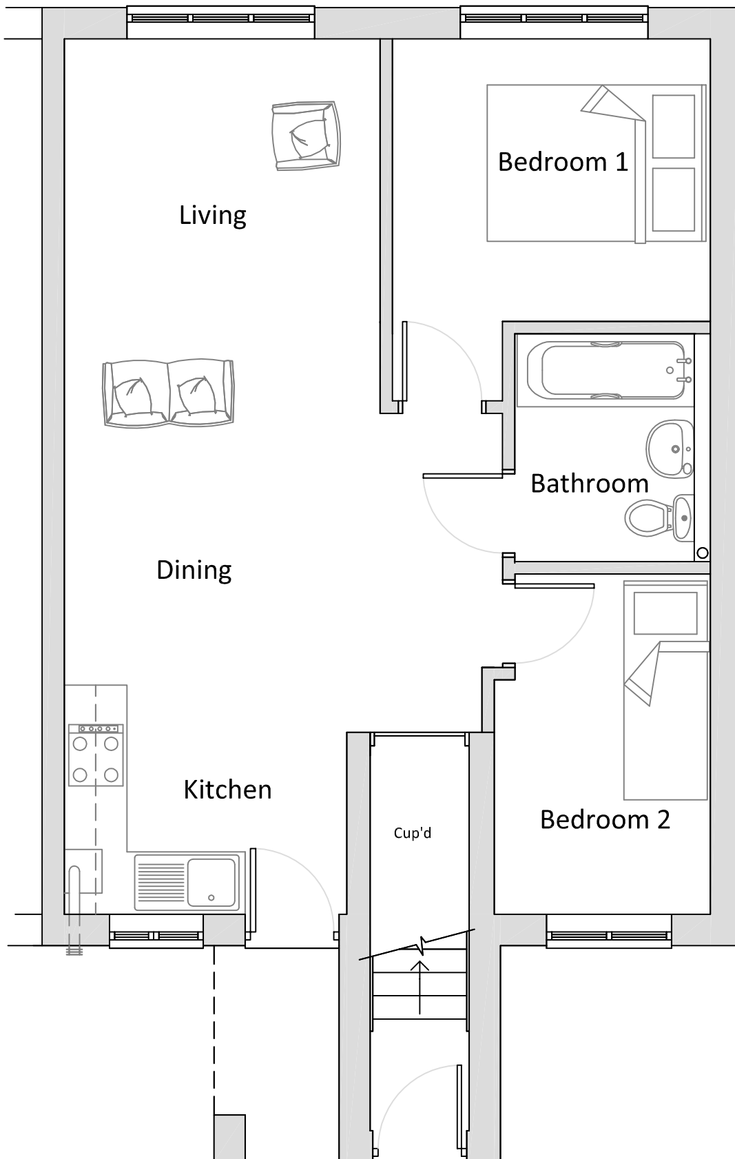
Ground Floor Layout Flat No 11
