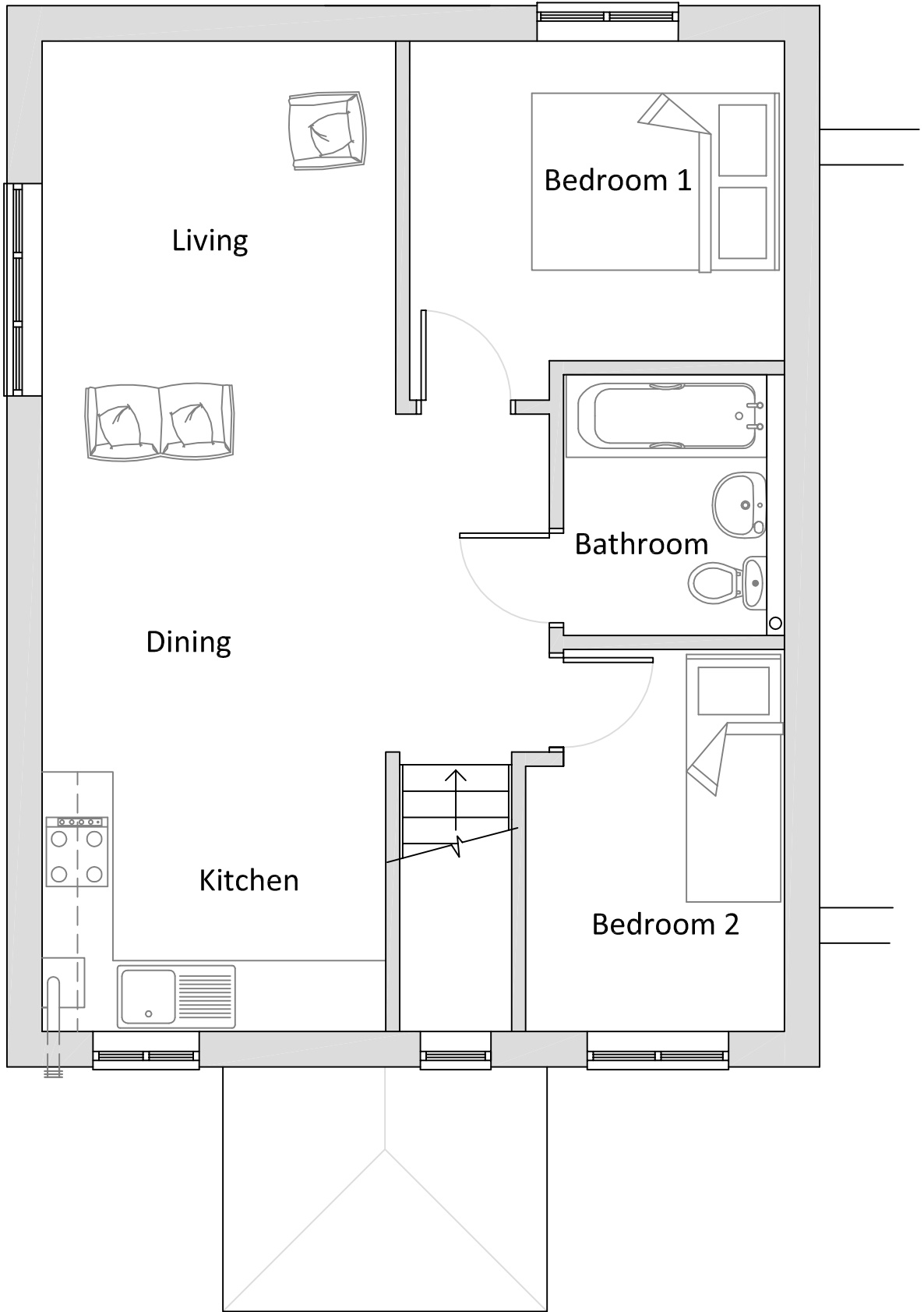
First Floor Layout Flat No 16
